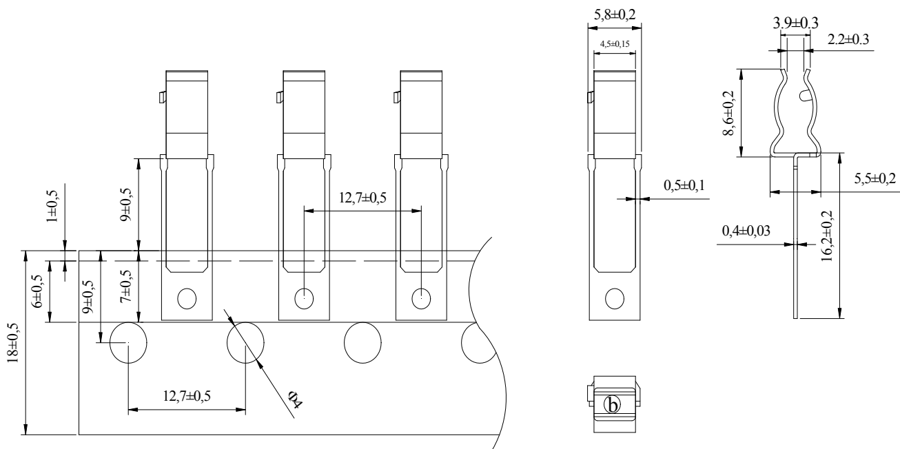
Dimensions (unit in mm)
