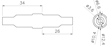
Dimensions (unit in mm)
