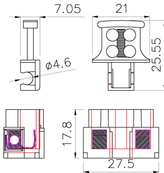
Dimensions (unit in mm)
