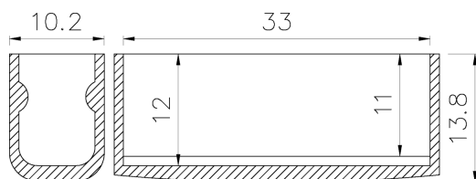
Dimensions (unit in mm)
