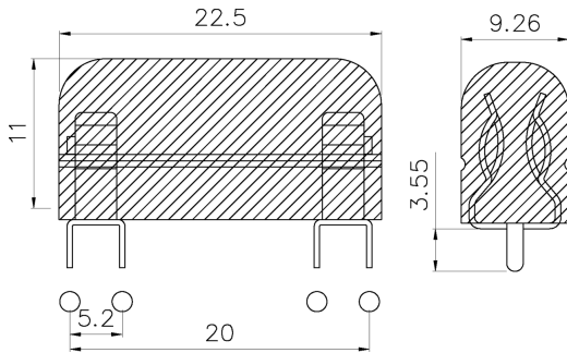
Dimensions (unit in mm)
