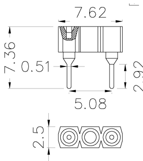
Dimensions (unit in mm)
