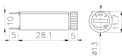
Dimensions (unit in mm)
