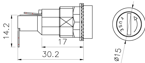
Dimensions (unit in mm)
