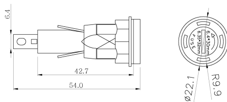
Dimensions (unit in mm)
